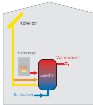
System B: 1-Speicher-System
